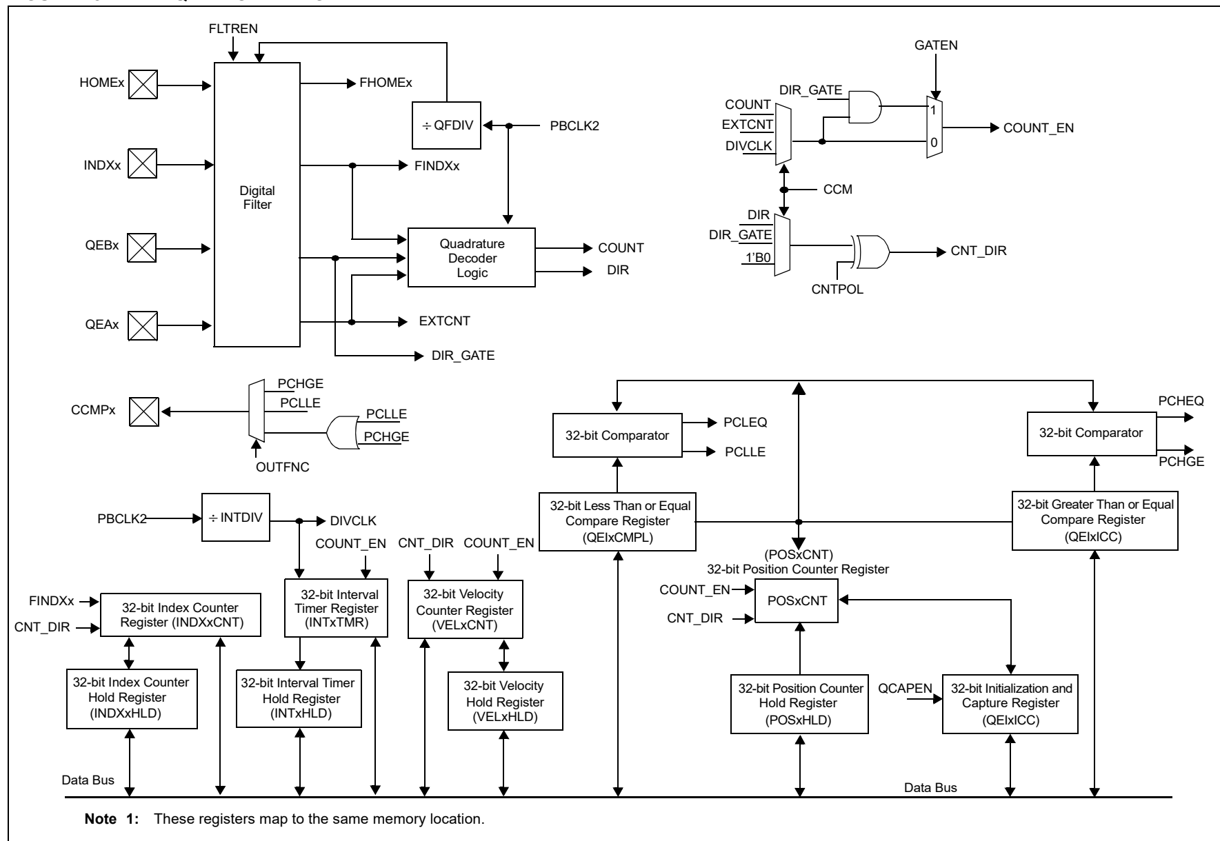
FIGURE 28-1: QEI BLOCK DIAGRAM
