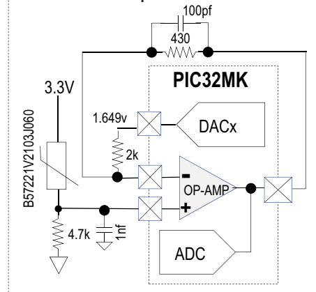
0-100°C NTC Temperature Sensor
