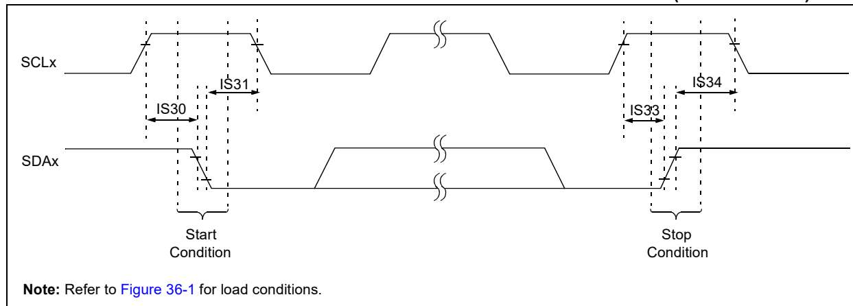
FIGURE 36-16: I2Cx BUS START/STOP BITS TIMING CHARACTERISTICS (CLIENT MODE)
