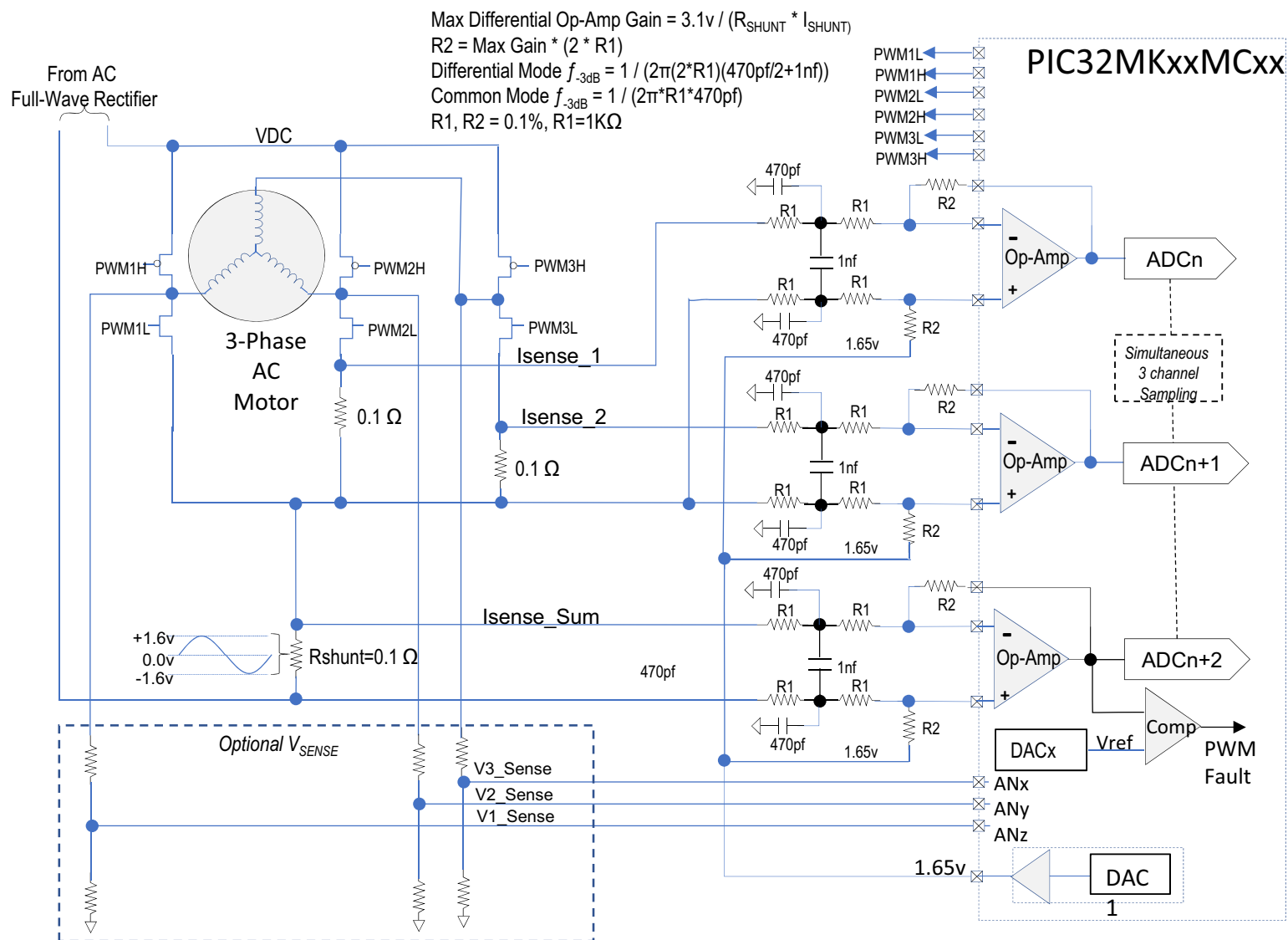
FIGURE 29-2: 3 PHASE AC MOTOR CONTROL EXAMPLE
