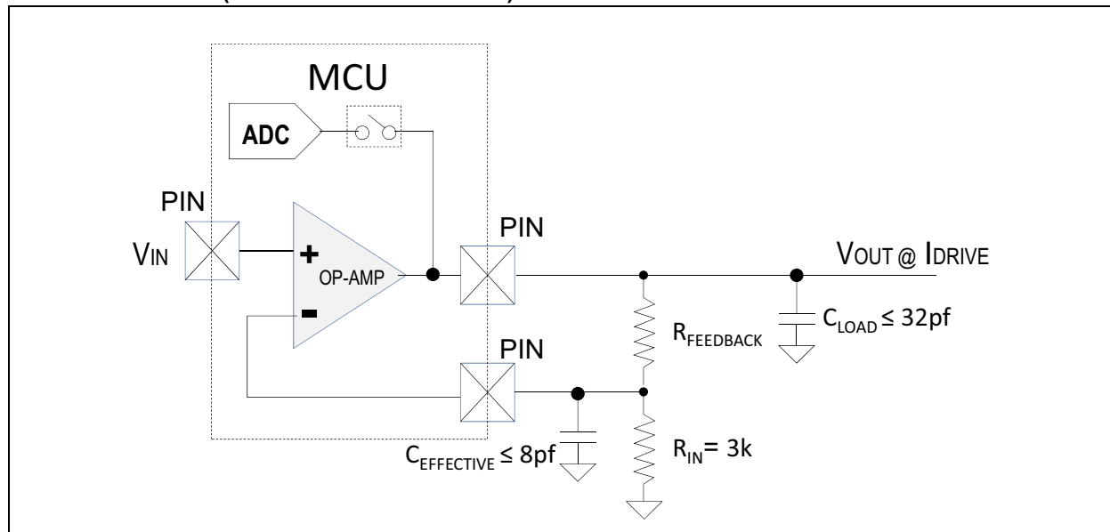
FIGURE 25-12: OP-AMP GAIN \geq 2 : LOW POWER MODE \leq 10\text{MHz} REQUIREMENTS (CMXCON<OPLPWR> = 1)
