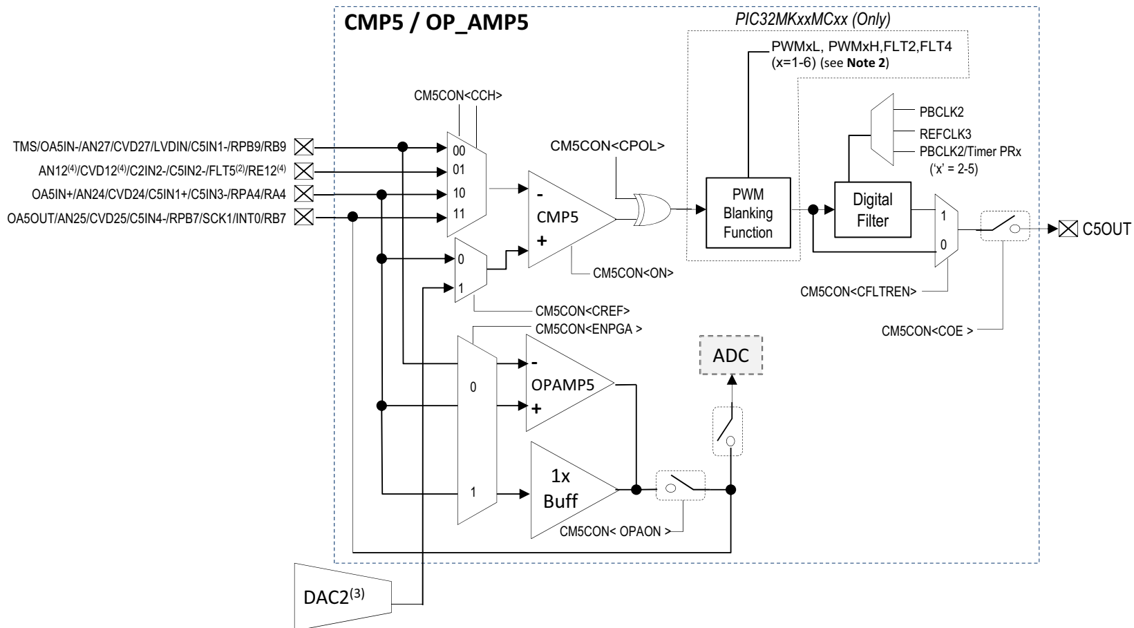
FIGURE 25-5: OP AMP 5/COMPARATOR 5 MODULE BLOCK DIAGRAM
