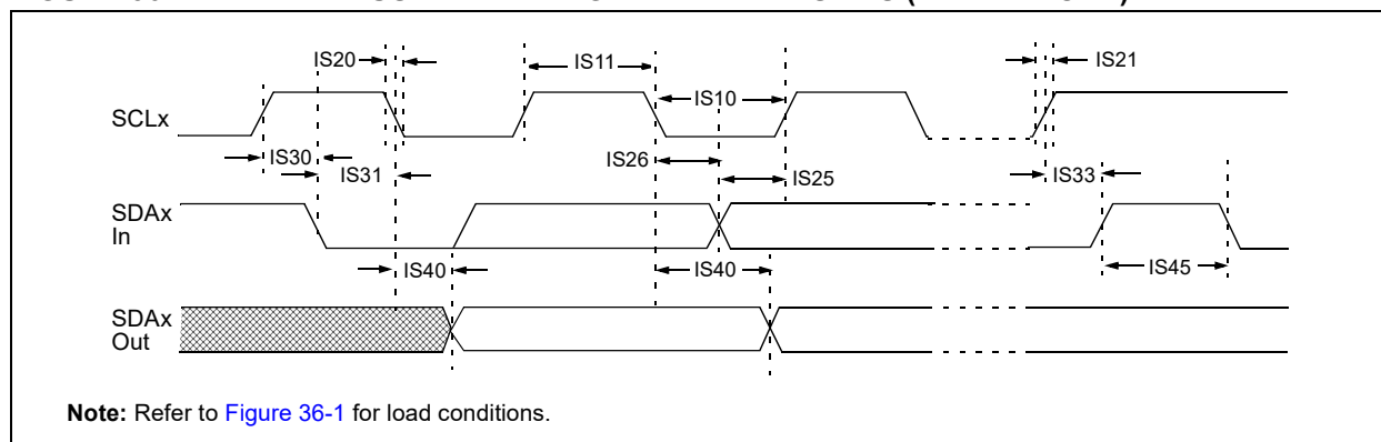
FIGURE 36-17: I2Cx BUS DATA TIMING CHARACTERISTICS (CLIENT MODE)
