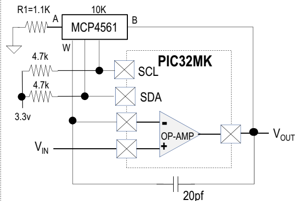
Programmable Gain Non-Inverting Amp (256 Steps)
